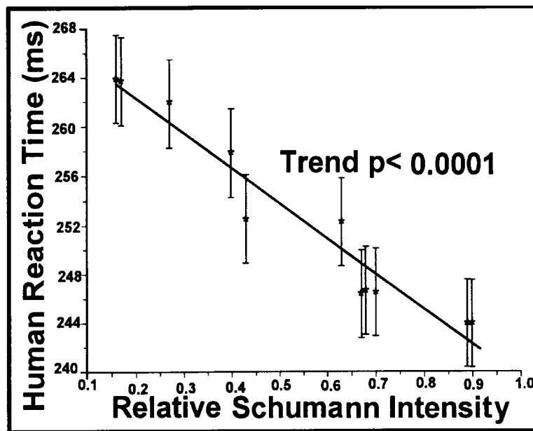
Figure 8. Human reaction times as a function of Schumann Resonance 8–10 Hz relative intensity. Reaction times measured using a light flash and a Morse key, tested during 18 days in September 1953, at the German Traffic exhibition in Munich.
