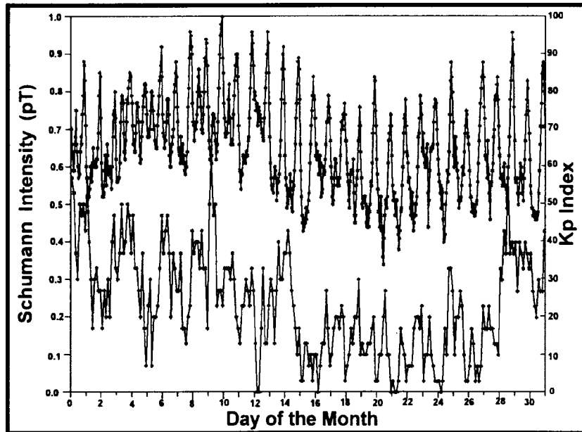
Figure 3. Schumann Intensity (0–20 Hz) from the UC Berkeley PKB site (upper graph) and Kp Index (lower graph) for March 1999.
