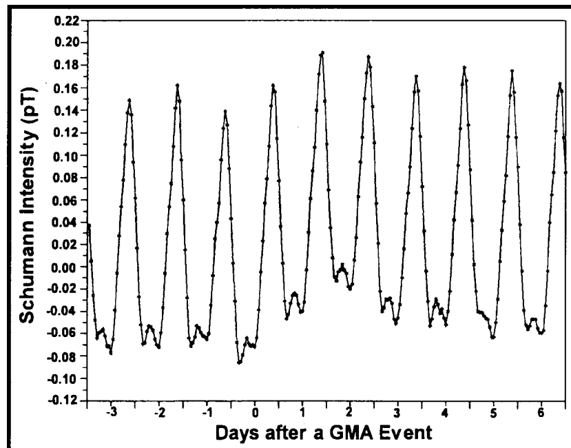
Figure 6. Superimposed epoch analysis of the impact of a Geomagnetic events, as defined by the Kp Index, for the mean anomaly in the Schumann Resonance 0–20 Hz intensity for 69 events in 1997 to 1999. GMA events occurred on day zero.
