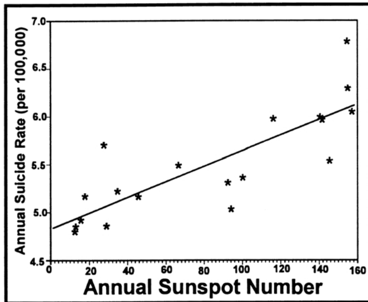
Figure 10. Annual male suicide rate per 100,000 for Thailand from 1974 to 1992, in relation to the annual sunspot number. The correlation coefficient is r = 0.817 , p < 0.0001 .
