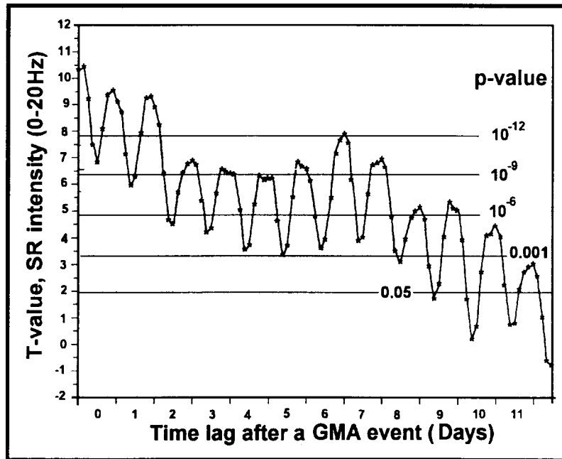
Figure 5. The statistical Student t-value of the time lagged correlation between the 3-hour Kp index and the 3-hr mean Schumann Resonance Intensity for the 0–20 Hz band, for the period September 1996 to December 1999.
