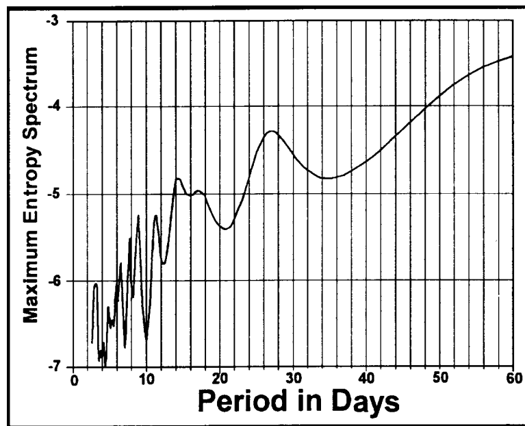
Figure 7. Maximum entropy spectrum for the 2-day average 0–20 Hz Schumann Resonance Intensity for the period February 1997 to December 1999.
