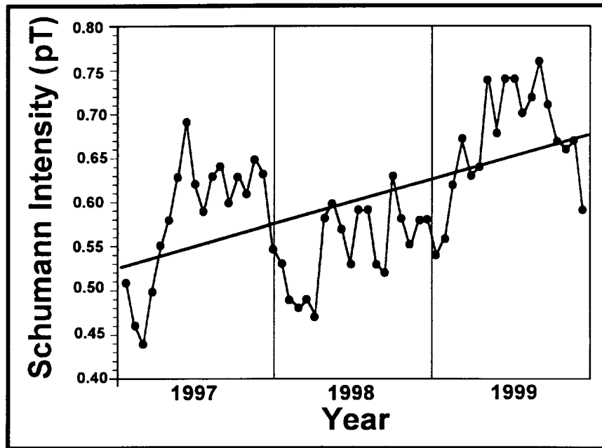
Figure 2. The time sequence of 20-day averaged Schumann Resonance signal intensity in the 0–20 Hz range. From the UC Berkeley dataset, for the three years used in this study. The trend is highly significant, p < 0.0001 .
