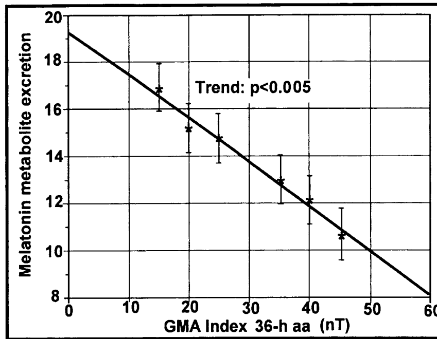
Figure 9. Reduction in the melatonin metabolite 6-OHMS in \mu\text{g} in urine from U.S. electric utility workers, as a function of the 36 hr global GMA aa-index (Burch et al. , 1999b).
